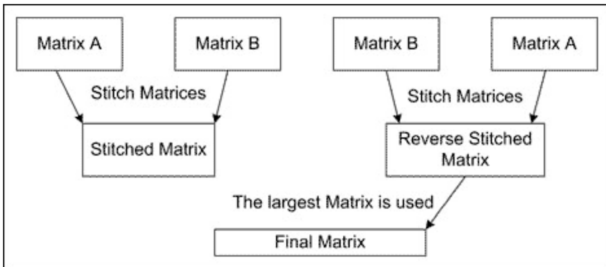
Figure 5. Reverse code stitching doubles processing time, often with minimal code gains.
