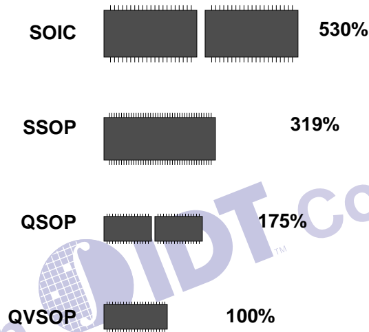
Figure 1. Relative Area of 16 Bit Packaging Solutions
